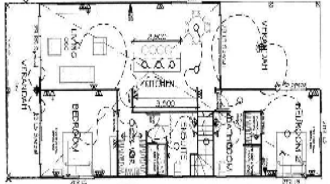
NEW 2 Bedroom Executive Villa Layout
